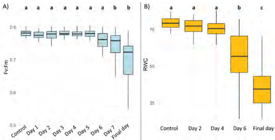
Figure 1: Perennial ryegrass drought stress response based on the maximum photochemical efficiency of photosystem II (Fv:Fm) (A) and leaf relative water content (RWC) (B). The letters indicate difference among group means (Tukey's HSD test, p < 0.005 ).
