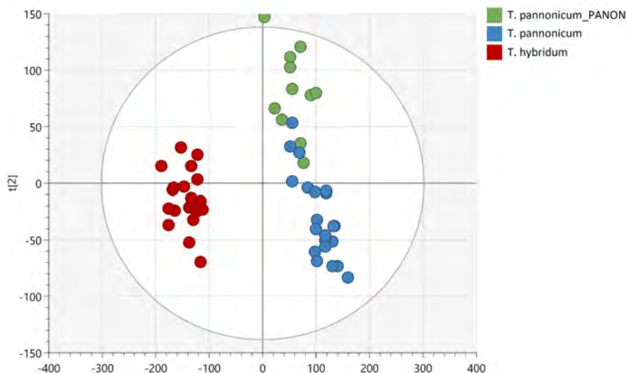
Figure1: PCA score plot of 1H NMR data from two Trifolium species: T. pannonicum , variety Panon, wild material and T. hybridum , variety K50.
