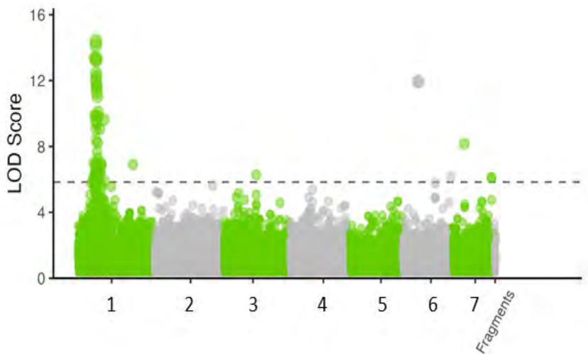
Figure 1: Hardseed Manhattan Plot
